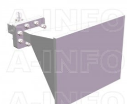
LB-137-15-C-TFSPO Standard Gain Horn Antenna 5.85-8.2GHz 15dB Gain TNC Female
