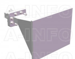
LB-137-15-C-SFSPO Standard Gain Horn Antenna 5.85-8.2GHz 15dB Gain SMA Female
