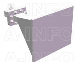
LB-137-15-C-NFSPO Standard Gain Horn Antenna 5.85-8.2GHz 15dB Gain N Type Female
