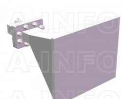
LB-137-15-C-3.5FSPO Standard Gain Horn Antenna 5.85-8.2GHz 15dB Gain 3.5mm Female
